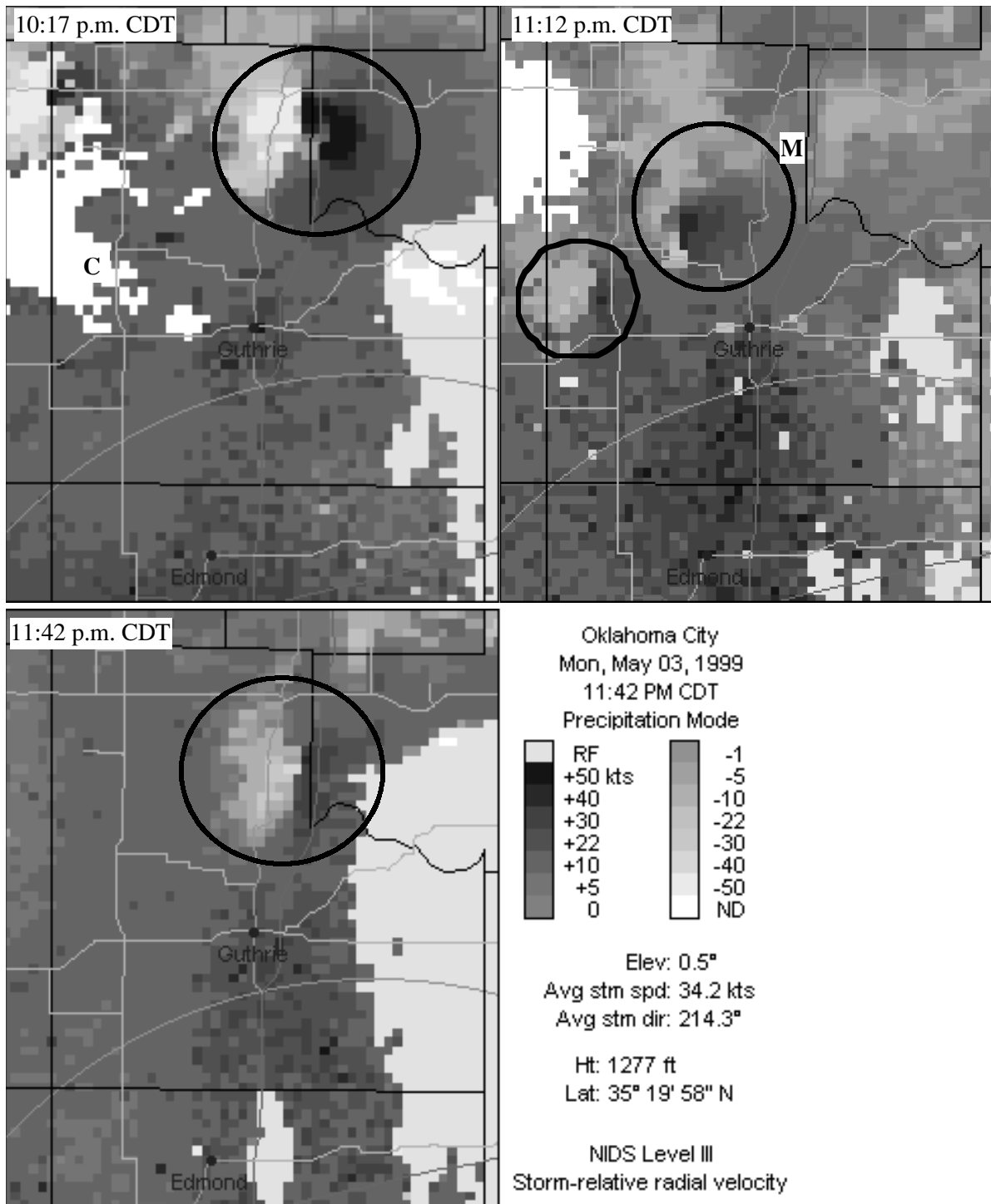
Figure 5. Gray-scale versions of storm-relative radial velocity from the Oklahoma City WSR-88D at 10:17 p.m., 11:12 p.m., and 11:42 p.m. local time. Circled areas were added for clarity in this manuscript to highlight tornadic supercell thunderstorms ( i.e. , radial velocity couplets). Light thin lines denote various highways. The circled storm at 10:17 first hit the Crescent area (marked by "C") and subsequently the town of Mulhall (denoted by "M"). Crescent was sandwiched between two tornadoes at 11:12 that followed similar tracks. The southwestern storm at 11:12 (just entering Logan County) was the same storm that was near the Mulhall area at 11:42. Color versions of these images were guidance for the decisions made by Logan County Emergency Management as discussed in the text.
