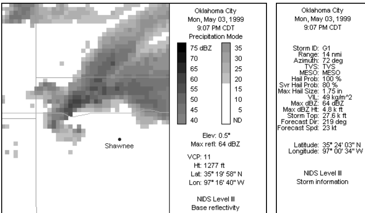
Figure 6. OK-FIRST images used by Seminole County Emergency Management to warn emergency vehicles. A hook echo in base reflectivity from the Oklahoma City WSR-88D at 9:07 p.m. local time (left) crosses interstate highway I-40, while a cursor read-out of storm attribute information (right) provides more detailed information.
