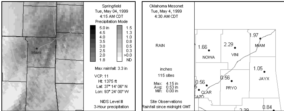
Figure 7. Three-hour rainfall accumulation from the Springfield WSR-88D radar at 4:15 a.m. local time, indicating more than 3 inches in Ottawa County near Miami (left) and total rainfall accumulations through 4:30 a.m. local time from the Oklahoma Mesonet (right). Corresponding flash food guidance values for Craig and Ottawa counties were 2.2 inches.
